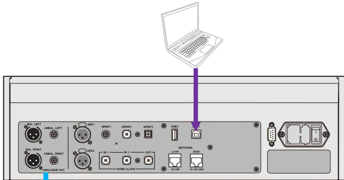
Figure 4 – Using a Rossini Player with a laptop
