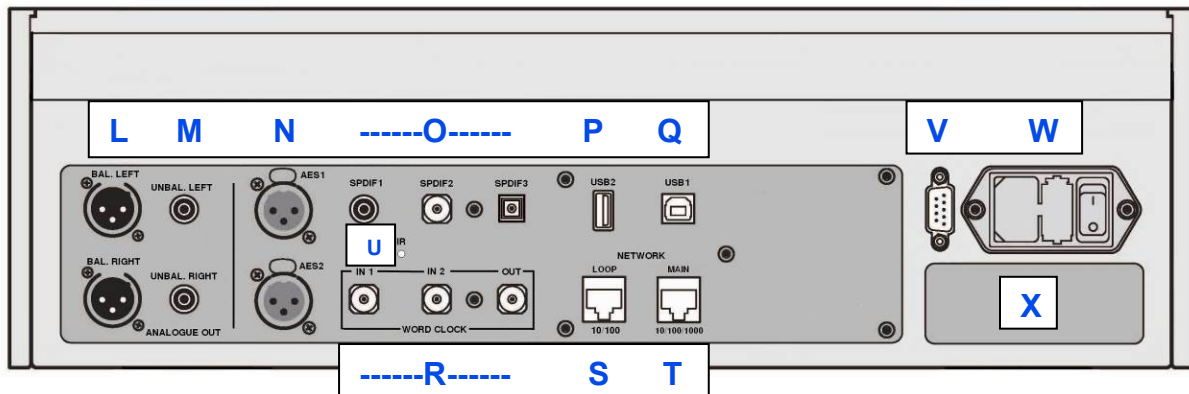
Figure 9 – Rear panel
