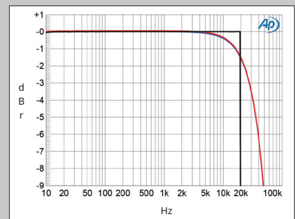
Fig.5 dCS Vivaldi Apex, F5, frequency response at –12dBFS into 100k ohms with data sampled at: 44.1kHz (left channel green, right gray) and 192kHz (left blue, right red) (1dB/vertical div.).
