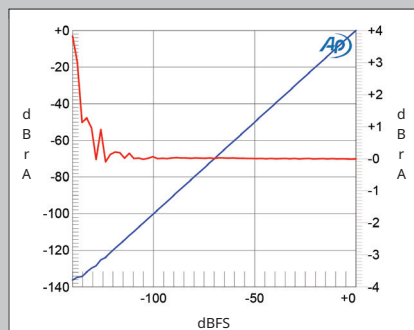
Fig.7 dCS Vivaldi Apex, Map 3, left channel, 1kHz output level vs 24-bit data level in dBFS (blue, 20dB/vertical div.); linearity error (red, 1dB/small vertical div.).
