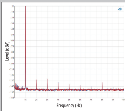
Fig.9 dCS Vivaldi Apex, balanced output, 24-bit data, spectrum of 1kHz sinewave, 10Hz-10kHz, at 0dBFS into 600 ohms (left channel blue, right red; linear frequency scale).
