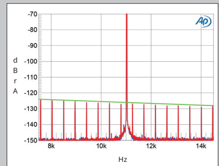
Fig.11 dCS Vivaldi Apex, high-resolution jitter spectrum of analog output signal, 11.025kHz at -6\text{dBFS} , sampled at 44.1kHz with LSB toggled at 229.6875Hz: 16-bit AES3 data (left channel blue, right red). Center frequency of trace, 11.025kHz; frequency range, \pm 3.5\text{kHz} .
